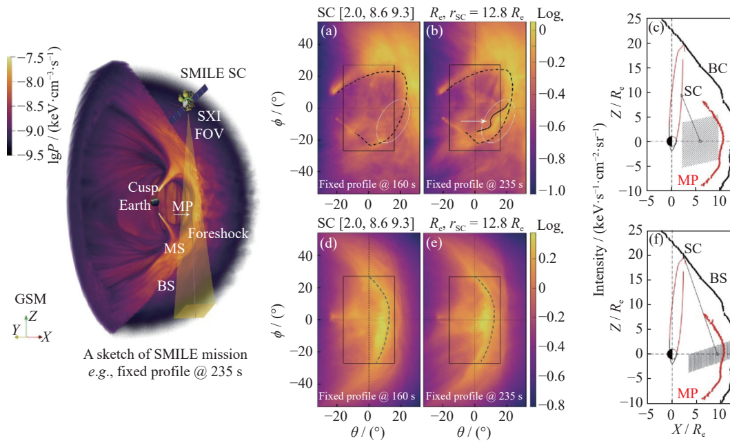
Fig. 3 Deformation of the magnetopause caused by high-speed jets as revealed by the X-ray emissivity (upper panel) and X-ray images (lower panel)
