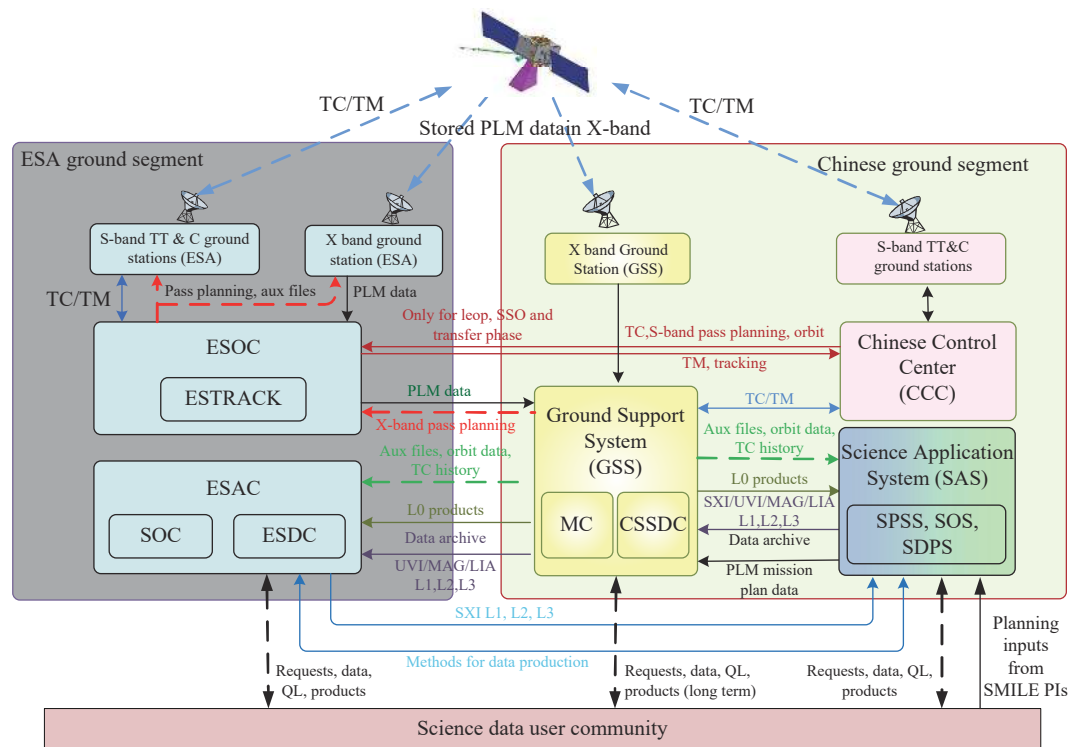
Fig. 9 SMILE ground segment architecture
