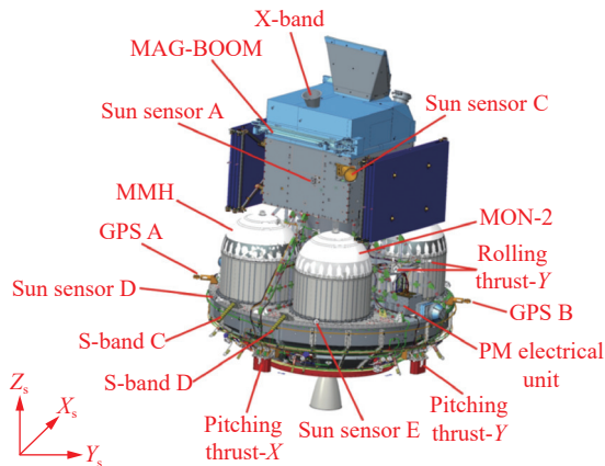
Fig. 1 SMILE satellite structure
