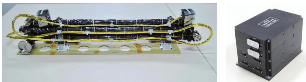
Fig. 7 FM of MAG boom (left) and electronic box (right)
