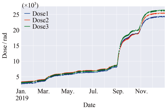
图1 2019年卫星舱内三个方向辐射剂量变化曲线 Fig.1 Radiation dose curve in three directions in satellite cabin in 2019
