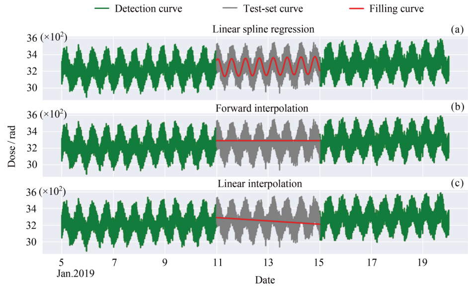
图 6 叠加正弦波的线性样条回归、前向插值、线性插值三种方法缺失值填充结果 Fig. 6 Result of sine-adjusted linear spline regression method, forward interpolation and linear interpolation
